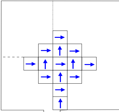
Parallel/chessboard-style installation of tiles
